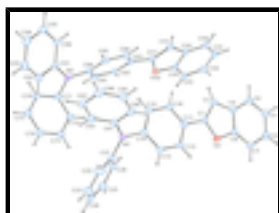
Fig. 1. Molecular structure of (I) with 30% probability displacement ellipsoids, showing the atom-numbering scheme employed. H atoms are shown as small spheres of the arbitrary radii.
